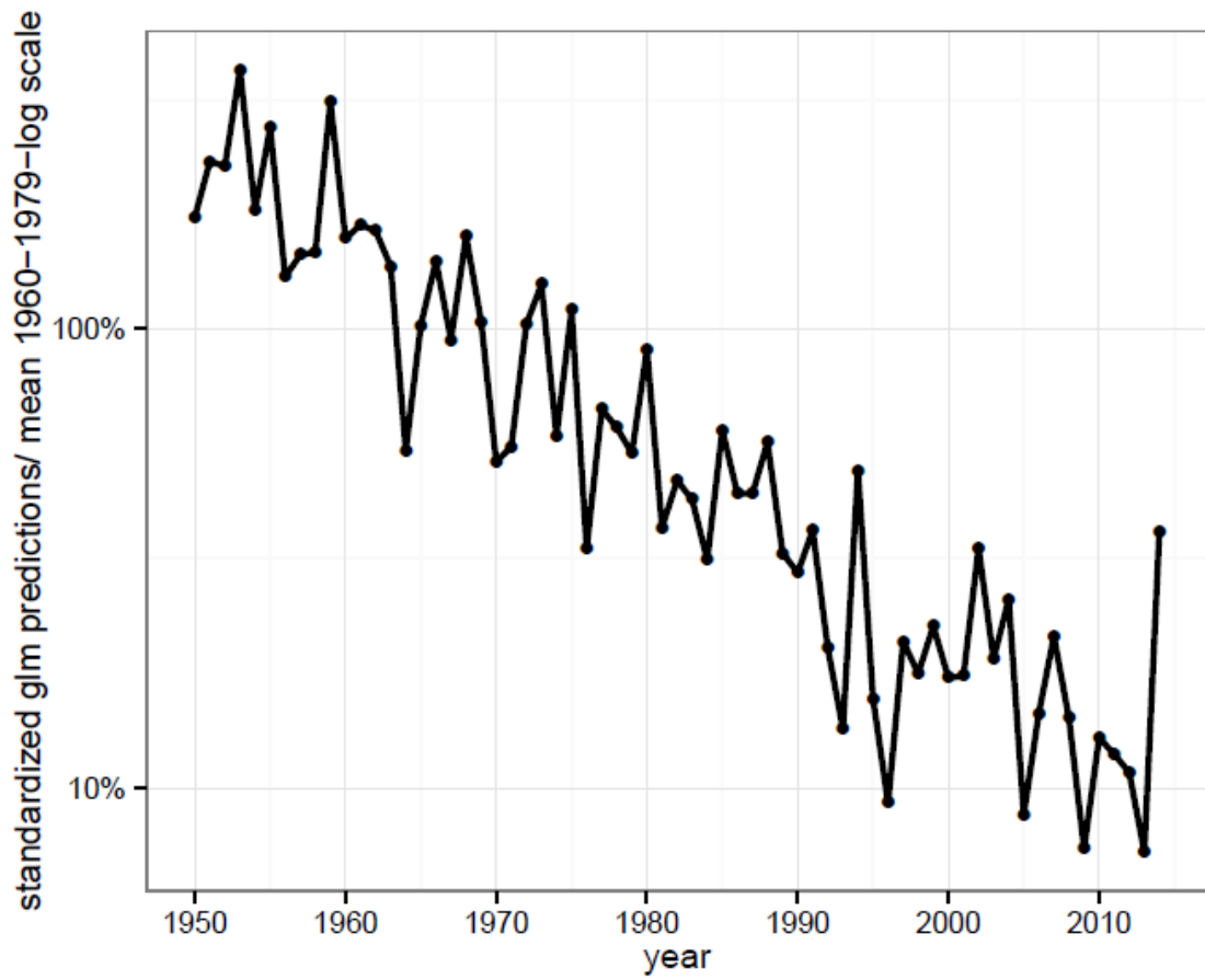
Figure 9.3.7.2 Mean of estimated (GLM) yellow eel recruitment and smoothed trends for Europe updated to 2014 (ICES, 2014. Note the logarithmic scale on the y-axis .
